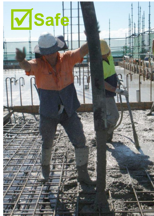
Figure 4 – Line hand guiding hose and signalling to pump operator.
